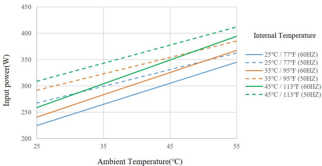
Power Consumption with Varied Temperature
