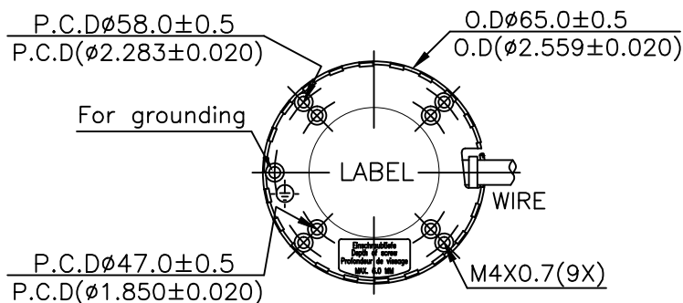
VIEW A of PILLOW
