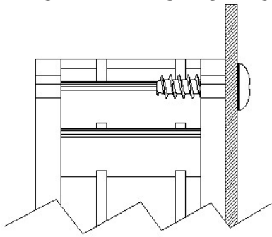
SELF-TAPPING SCREW FLANGE MOUNTING DRAWING
