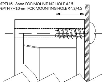
SELF-TAPPING SCREW RIB MOUNTING DRAWING
