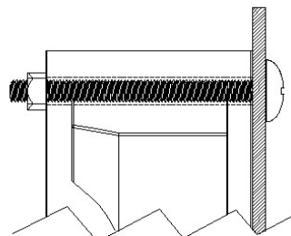
MECHANICAL SCREW RIB MOUNTING DRAWING
