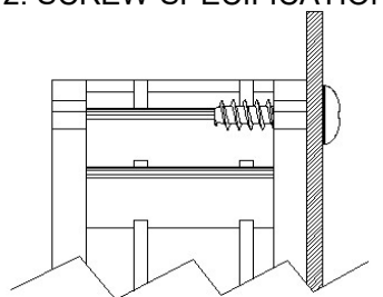
SELF-TAPPING SCREW FLANGE MOUNTING DRAWING
